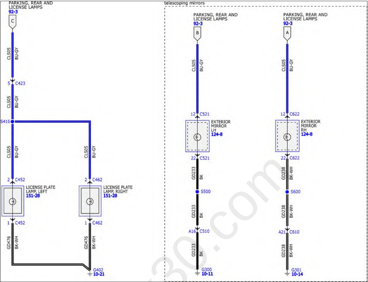
Fig 7: Parking Lamps, Rear Lamps and License Lamps System Wiring Diagrams (7 Of 7)
