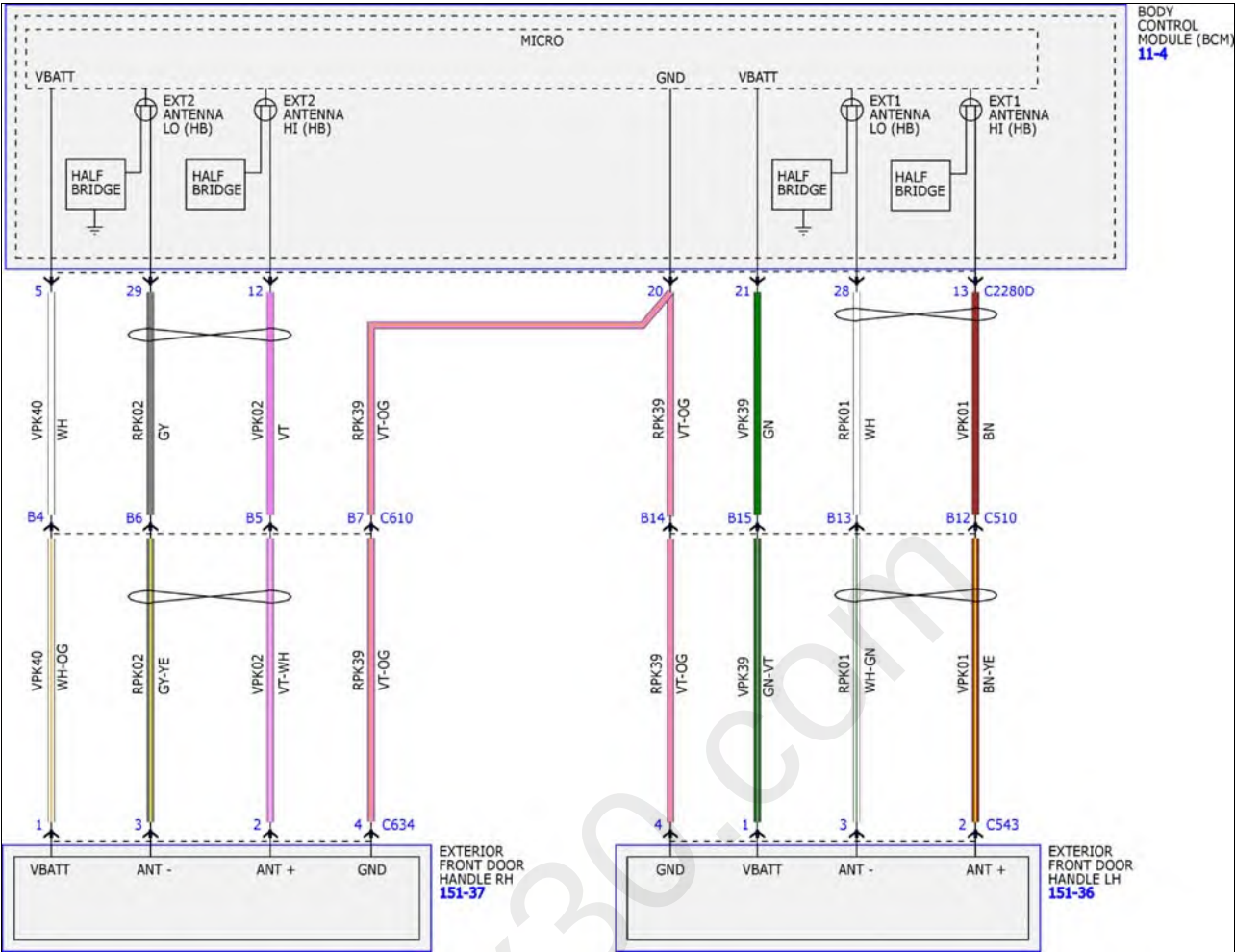
Fig 2: Passive Anti-Theft System Wiring Diagrams (2 Of 5)
