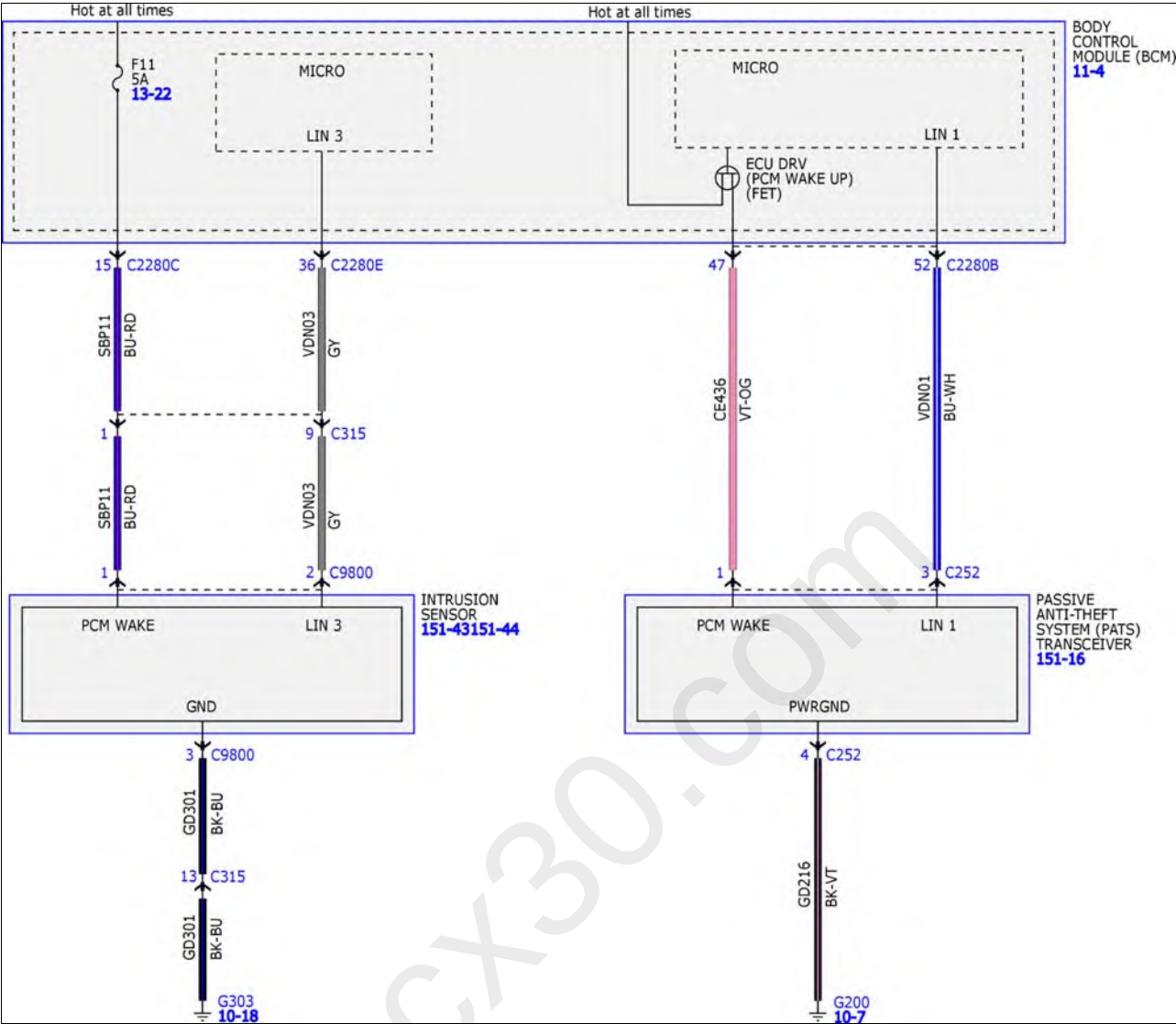
Fig 4: Passive Anti-Theft System Wiring Diagrams (4 Of 5)
