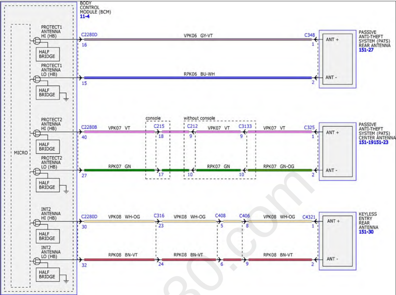
Fig 3: Passive Anti-Theft System Wiring Diagrams (3 Of 5)
